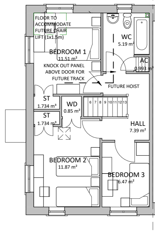
FIRST FLOOR PLAN - SIDE FRONTAGE 1 : 100
