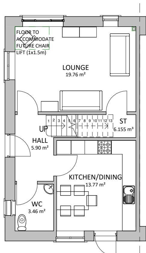
GROUND FLOOR PLAN - FRONT FRONTAGE 1 : 100
