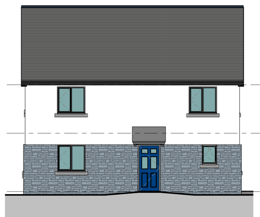
FRONT FRONTAGE SIDE ELEVATION 1 : 100 PLOT 6
