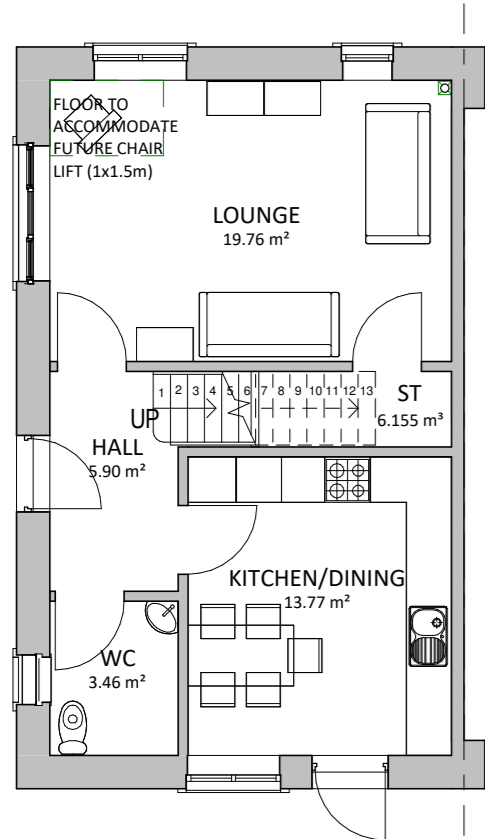
GROUND FLOOR PLAN - SIDE FRONTAGE 1 : 100
