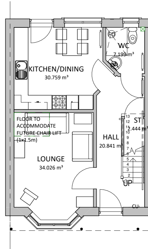
GROUND FLOOR PLAN - END TERRACE 1 : 100
