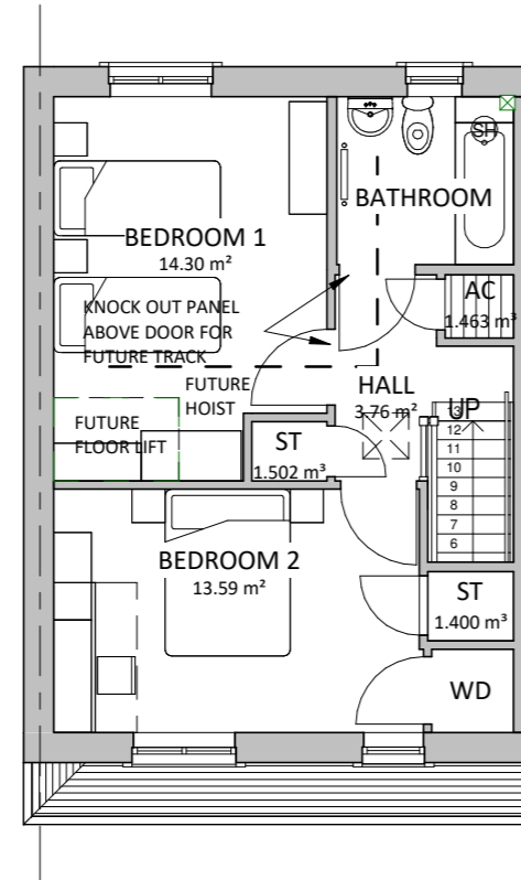
FIRST FLOOR PLAN - END TERRACE 1 : 100
